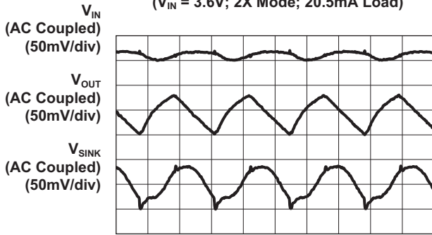
Output Ripple Waveform (VIN = 3.6V; 2X Mode; 20.5mA Load)
