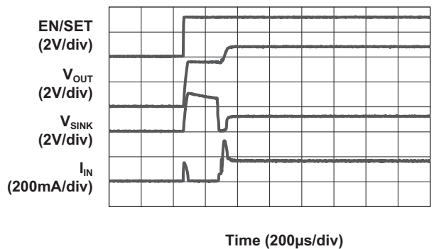
Turn On to 2X Mode ( V_{IN} = 3.6V ; 20.5mA/ch )
