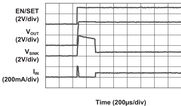
Turn On to 1X Mode ( V_{IN} = 4.2V ; 20.5mA/ch )
