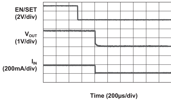
Turn Off from 2X Mode (20.5mA/ch)
